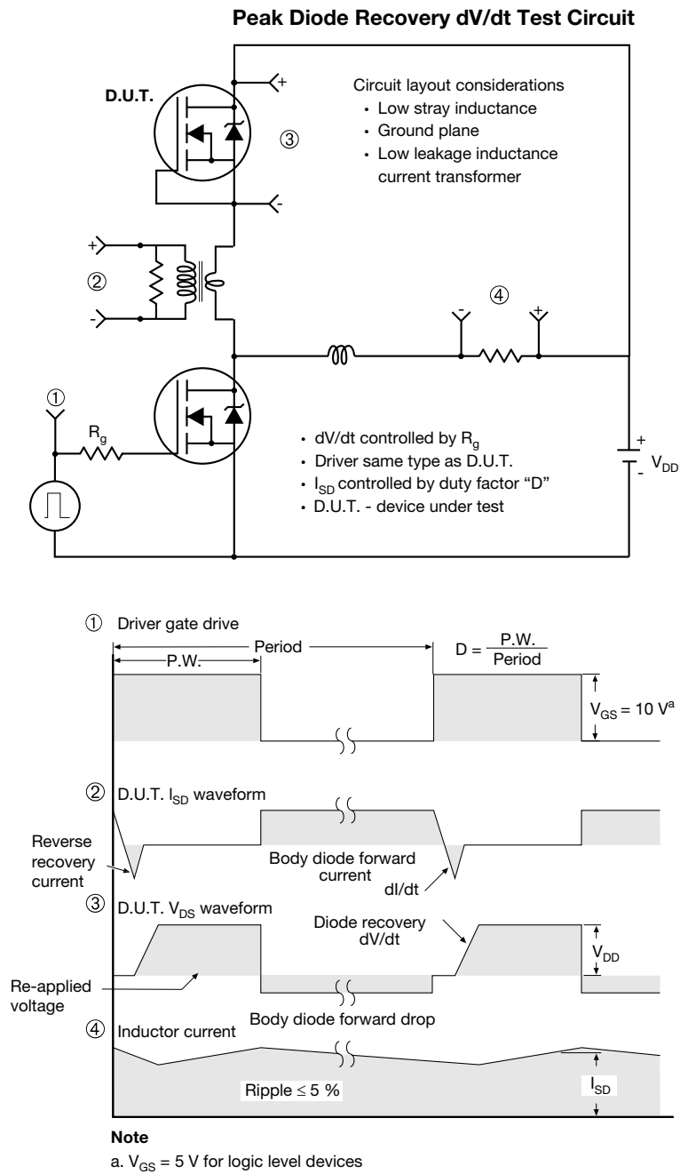
Fig. 19 - For N-Channel
